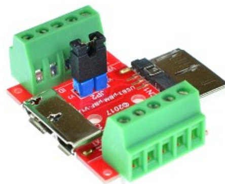
Figure 4: USB3-uBM-uBF-V1A with terminal blocks
